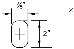
BOLT SLOT DETAIL (TYPICAL)
